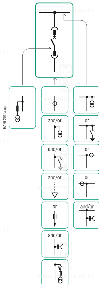
Circuit-breaker panel
