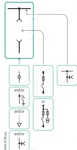
Vacuum contactor panel
