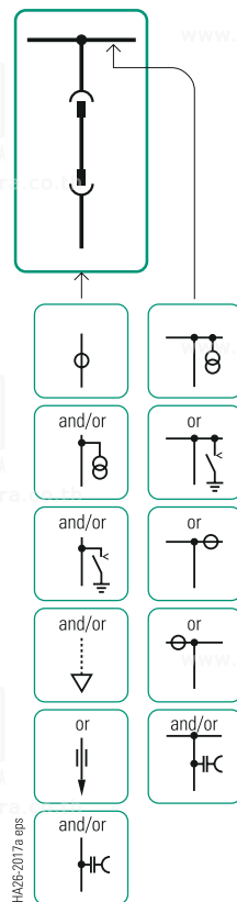
Disconnecting panel
